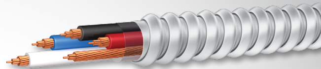
MC Feeder - THWN-2 Inners Available in sizes up to 750 KCMIL-4 conductor
