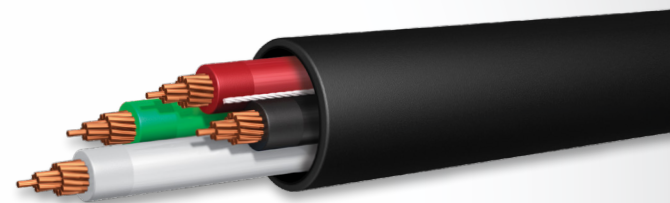
Tray Cable - Power and Control Cable - with or without Ground - THWN-2/XHHW-2 Inners Copper conductors available in 14 AWG-2 through 750 KCMIL-4, Aluminum conductors available in 6 AWG and larger
