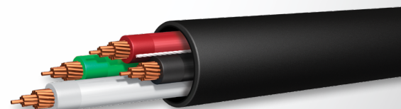
Tray Cable - Power and Control Cable - with or without Ground - THWN-2/XHHW-2 Inners Copper conductors available in 14 AWG-2 through 750 KCMIL-4, Aluminum conductors available in 6 AWG and larger
