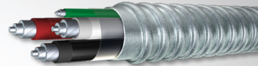
MC ALUMINUM CONDUCTORS - THWN-2 Inners Available in sizes up to 750 KCMIL-4 Conductor
