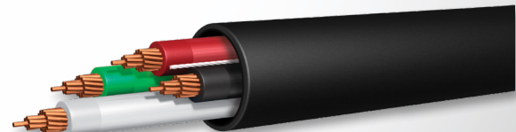
Tray Cable - Power and Control Cable - with or without Ground - THWN-2/XHHW-2 Inners Copper conductors available in 14 AWG-2 through 750 KCMIL-4, Aluminum conductors available in 6 AWG and larger
