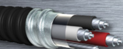
PVC Jacketed MC Cable with XHHW-2 Inners Available in Steel or Aluminum Armor
