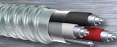
MC Cable with XHHW-2 Inners Available in Steel or Aluminum Armor
