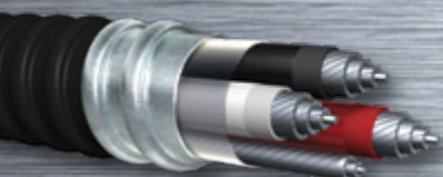
PVC Jacketed MC Cable with THHN/THWN-2 Inners Available in Steel or Aluminum Armor
