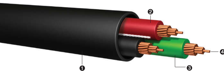
TYPE TC - Power Cable - Insulated Ground - XHHW-2 Inners
