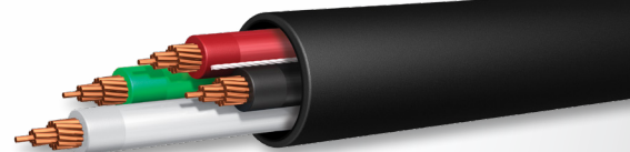
Tray Cable - Power and Control Cable - with or without Ground - THWN-2/XHHW-2 Inners Copper conductors available in 14 AWG-2 through 750 KCMIL-4, Aluminum conductors available in 6 AWG and larger
