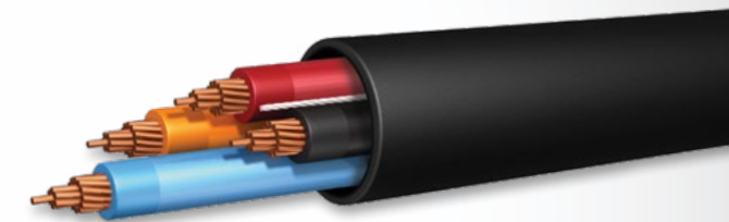
Tray Cable - Power and Control Cable - with or without Ground - THHN/XHHW-2/RW90 Inners Copper conductors available in 14 AWG-2 through 750 KCMIL-4, Aluminum conductors available in 6 AWG and larger
