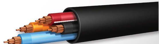
Tray Cable - Power and Control Cable - with or without Ground - THHN/XHHW-2/RW90 Inners Copper conductors available in 14 AWG-2 through 750 KCMIL-4, Aluminum conductors available in 6 AWG and larger
